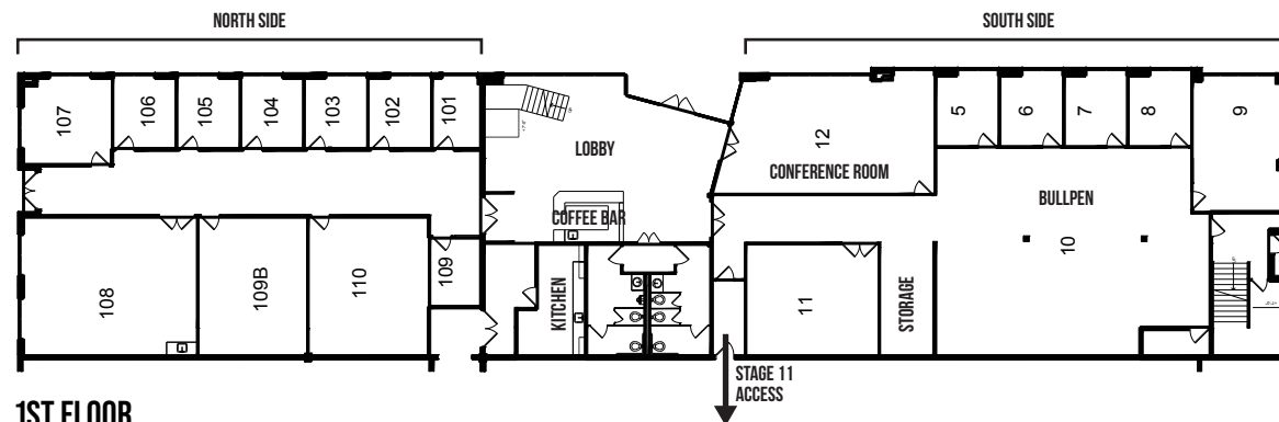
1ST FLOOR
